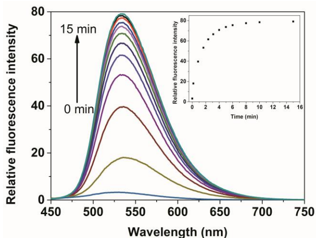
Figure 1. Fluorescence changes of sensor 1 (10 \mu M) upon addition of 10 equiv. of HS - in HEPES buffer solution (pH 7.4, 20 mM). Spectra were collected for 0 to 15 min at 25 °C with excitation at 435 nm. The inset shows a time course of the fluorescence intensity change.
