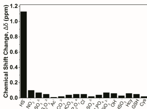
Figure 3. ^{129}\text{Xe} NMR chemical shift change of sensor 1 (100 \mu\text{M} ) after addition of 10 equiv. various other species (except for Cys, which is 4 equivalent) for 10 min. Bars represent the value of the ^{129}\text{Xe} chemical shift in the presence of various other species relative to the ^{129}\text{Xe} chemical shift of sensor 1. All the spectra were obtained with two scans under the conditions of 20 mM HEPES (pH 7.4) buffer with 60% DMSO as cosolvent at 25 ^{\circ}\text{C} .
