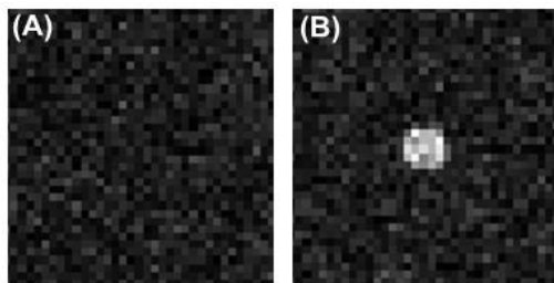
Figure 4. ^{129}\text{Xe} axial gradient-echo MRI images of a 10 mm tube containing (A) 100 \mu\text{M} sensor 1 and (B) 100 \mu\text{M} sensor 1 treated with 10 equiv. \text{HS}^- for 10 min under the test conditions. Images were acquired with a soft radiofrequency pulse centered at \delta = 74.1 ppm.
