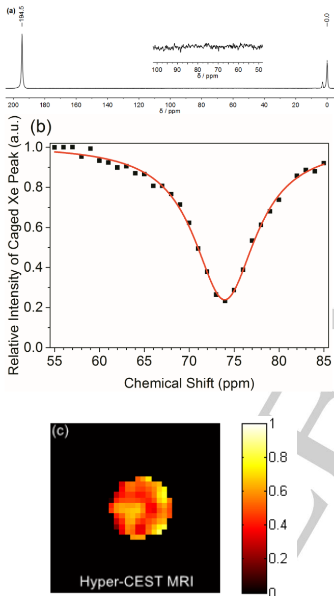
Figure 6. (a) 129 Xe NMR spectrum of sensor 1 labeled A549 cells (treated with 200 μM NaHS for 0.5 h then incubated with 25 μM sensor 1 for another 2 h) obtained by 4096 signal averages. (b) Hyper-CEST spectra of sensor 1 labeled A549 cells (treated with 200 μM NaHS for 0.5 h then incubated with 25 μM sensor 1 for another 2 h). Exponential fit (red solid line). (c) MRI of Hyper-CEST effect. The Hyper-CEST effect was calculated by using the formula CEST effect = (offRes - onRes) / offRes.
