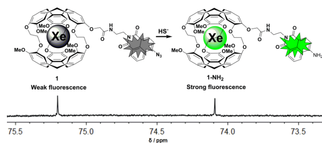
Scheme 1. Schematic of ^{129}\text{Xe} MRI sensor 1 for \text{H}_2\text{S} detection and imaging.
