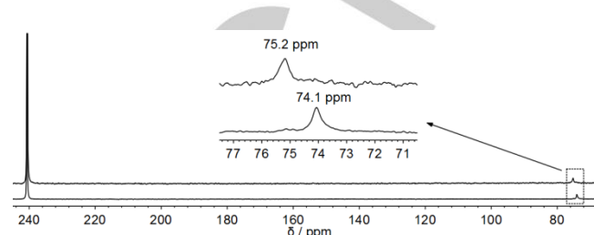
Figure 2. 129 Xe NMR spectrum change of sensor 1 (100 μM) upon addition of 10 equiv. of HS - . The spectra were obtained with two scans under the conditions of 20 mM HEPES (pH 7.4) buffer with 60% DMSO as cosolvent at 25 °C. The inset was the enlarged regional spectra.
