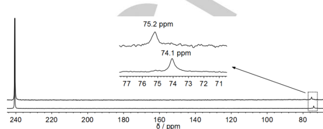
Figure 2. 129 Xe NMR spectrum change of sensor 1 (100 \mu M) upon addition of 10 equiv. of HS - . The spectra were obtained with two scans under the conditions of 20 mM HEPES (pH 7.4) buffer with 60% DMSO as cosolvent at 25 °C. The inset was the enlarged regional spectra.
