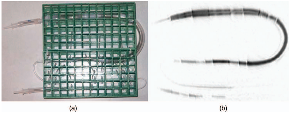
FIG. 3. The tubes phantom. (a) Digital photograph, (b) HP ^3\text{He} MR projection negative.
