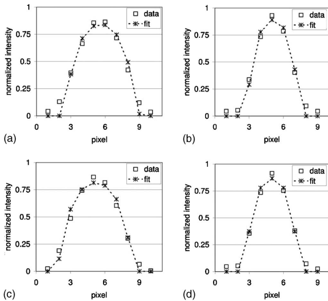
FIG. 6. Imaged pixel intensity profiles and their corresponding model-based fits. (a) Tube 3, Magnevist-filled, (b) tube 4, Magnevist-filled, (c) tube 3, HP ^3\text{He} -filled, (d) tube 4, HP ^3\text{He} -filled.
