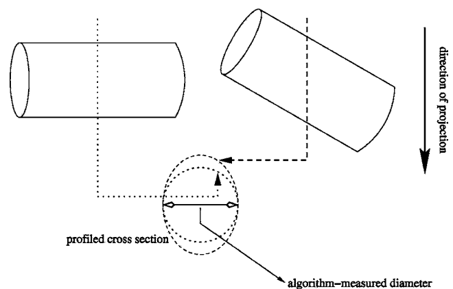
FIG. 9. Projected tube sections with and without inclination; a projection through the tube that is perpendicular to the projection direction (dotted line) intersects a circular section (dotted circle); a projection through the tube tilted with respect to the projection direction (dashed line) intersects an elliptical section (dashed circle).
